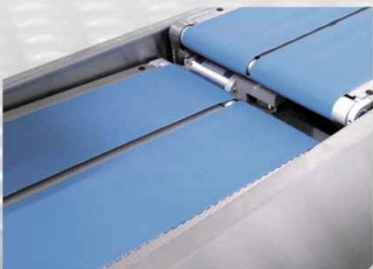
Labelling conveyor with lowering device for long packages, user-friendly with quick changeover.
