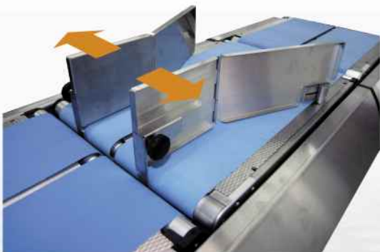
Automatic adjustment of alignment station.
