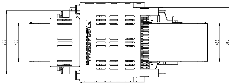
1800 BELT LENGTH VERSION
